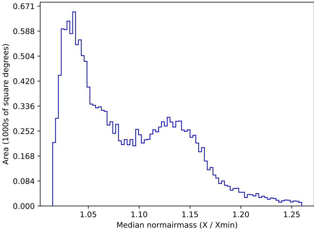
too_elab_r16_d3_giz_v3.4_10yrs WFD g band: Median normairmass
