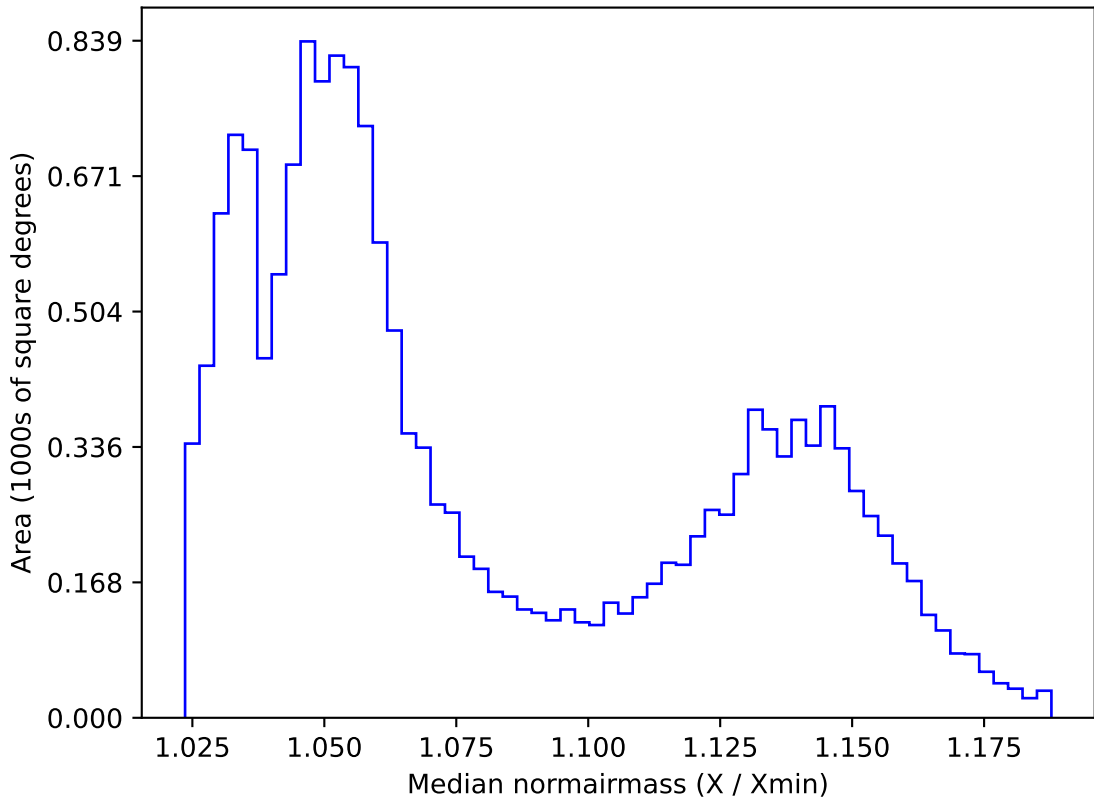
too_elab_r16_d3_giz_v3.4_10yrs WFD all bands: Median normairmass
