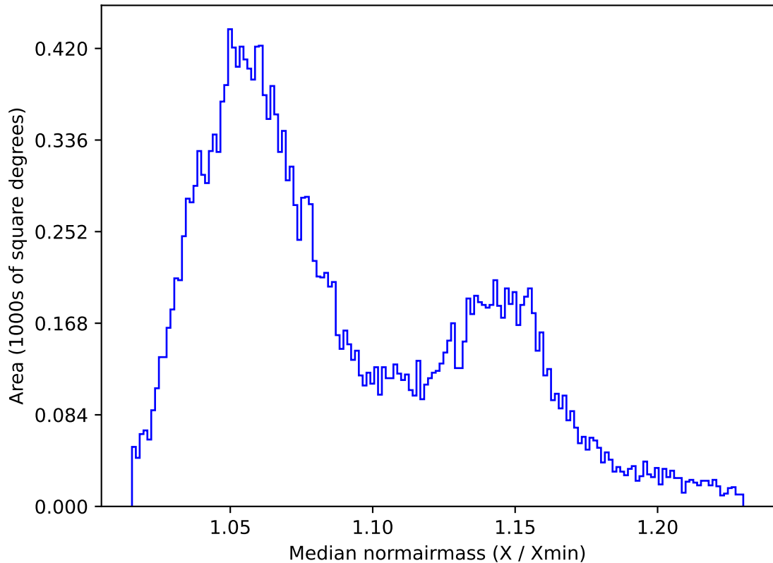
too_elab_r16_d3_giz_v3.4_10yrs All sky y band: Median normairmass
