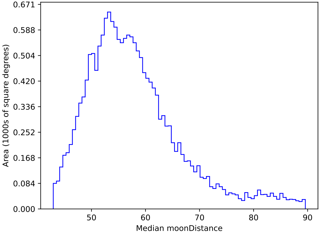
too_elab_r16_d3_giz_v3.4_10yrs WFD y band: Median moonDistance
