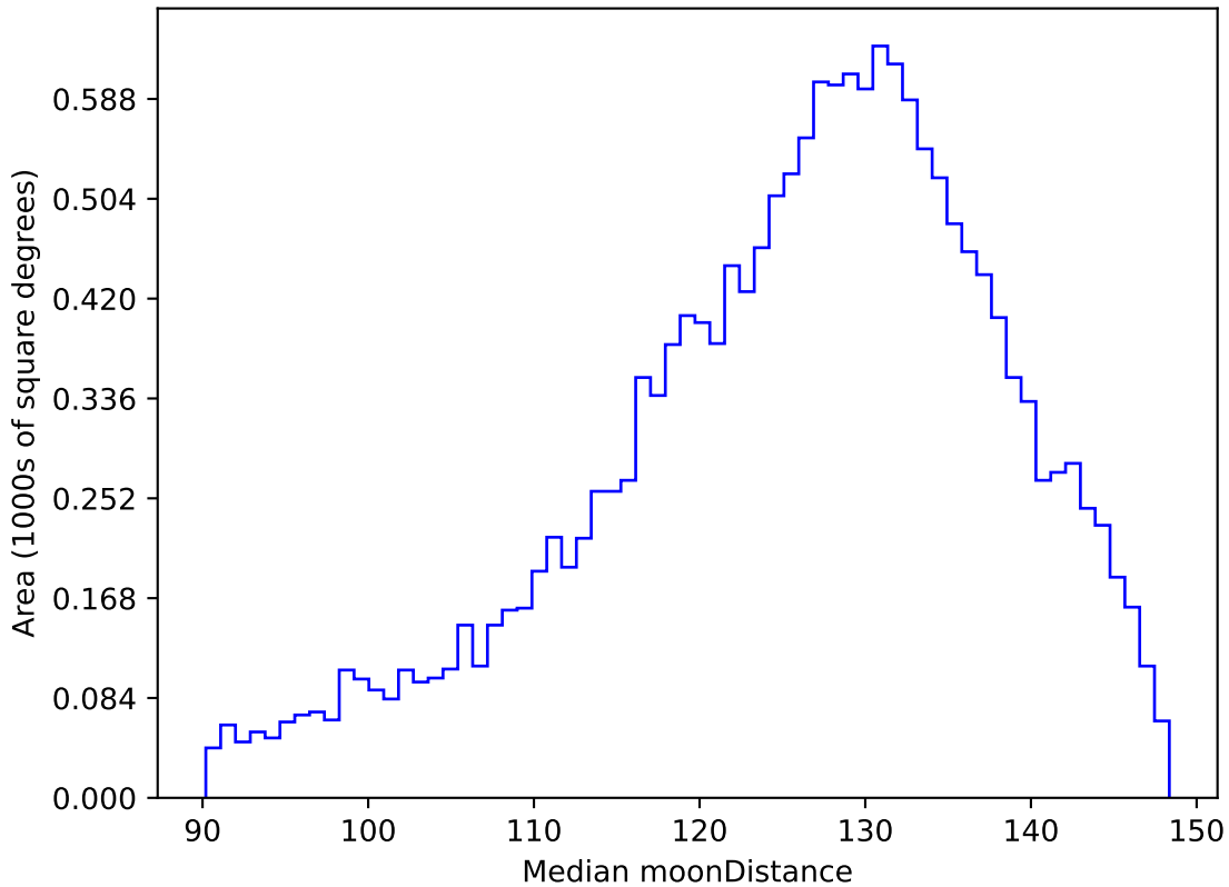
too_elab_r16_d3_giz_v3.4_10yrs WFD u band: Median moonDistance
