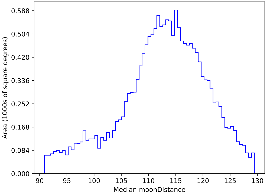
too_elab_r16_d3_giz_v3.4_10yrs WFD r band: Median moonDistance
