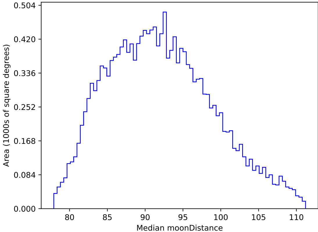
too_elab_r16_d3_giz_v3.4_10yrs WFD i band: Median moonDistance
