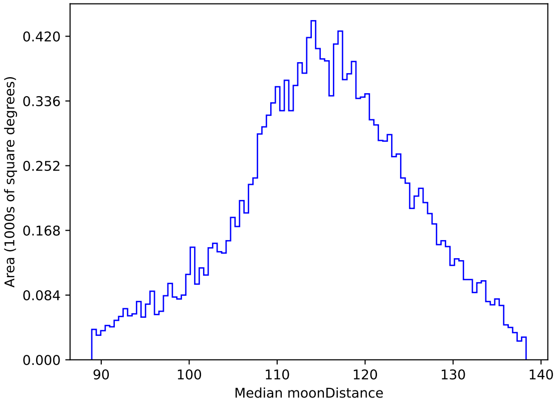
too_elab_r16_d3_giz_v3.4_10yrs WFD g band: Median moonDistance
