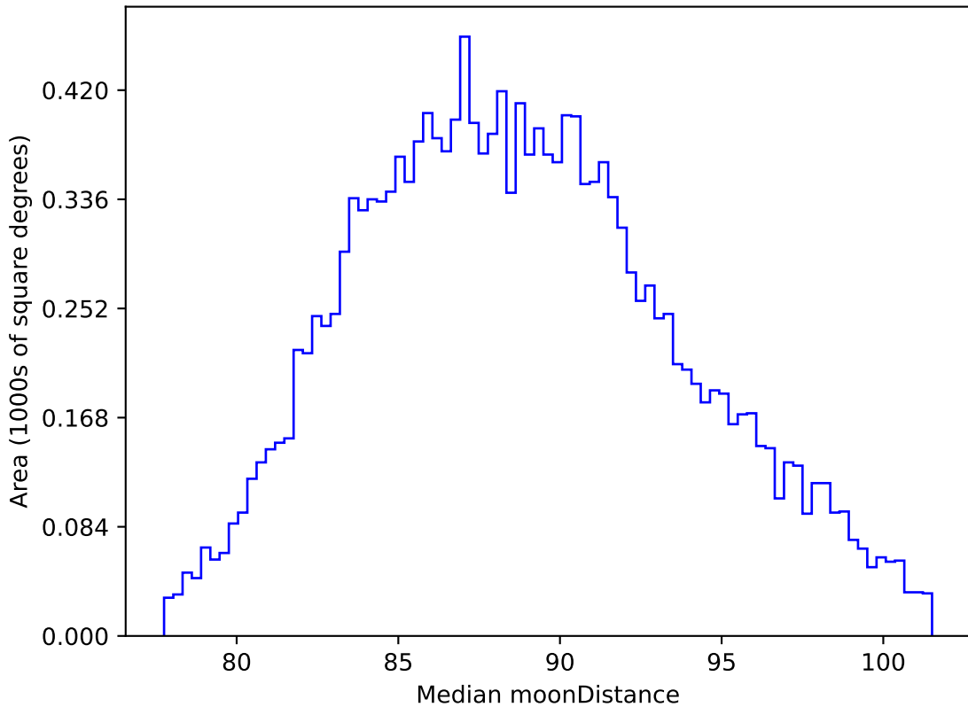
too_elab_r16_d3_giz_v3.4_10yrs WFD all bands: Median moonDistance
