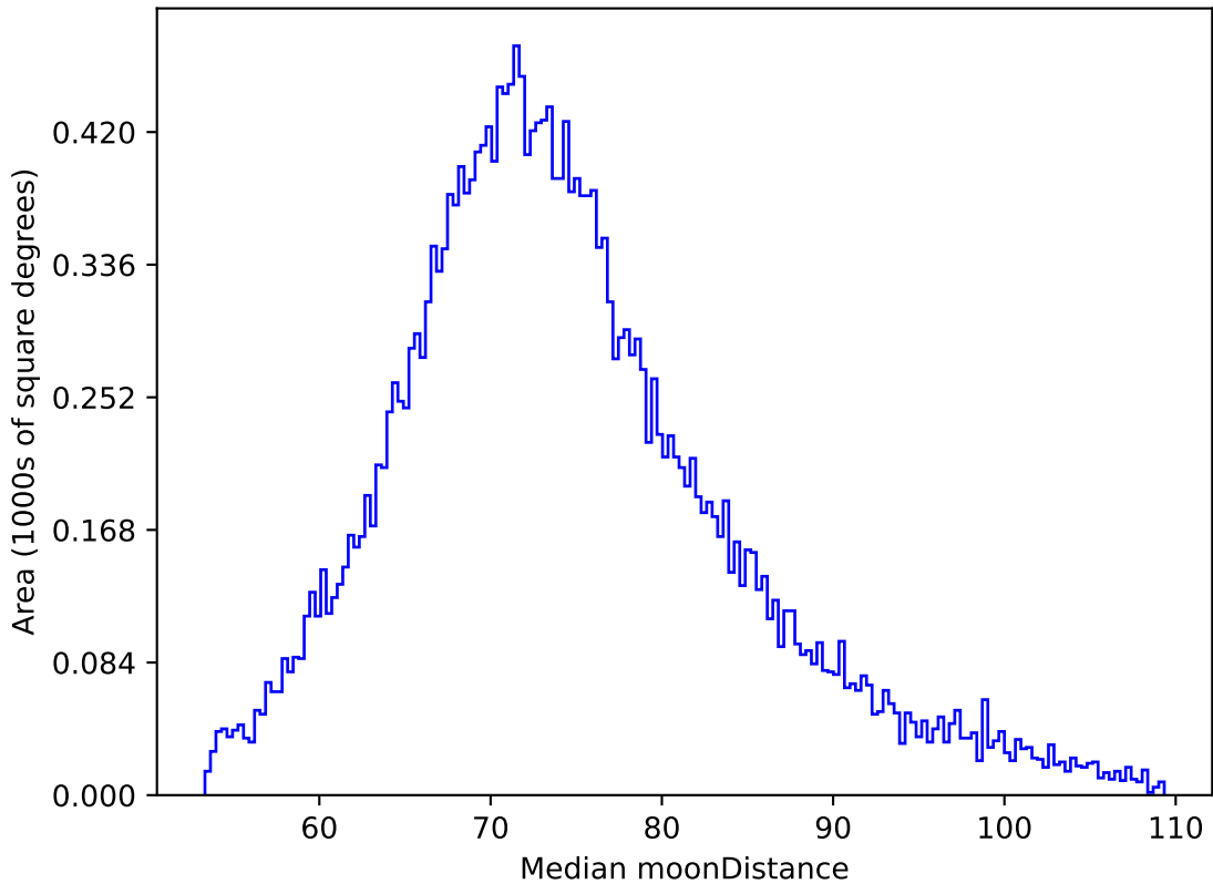
too_elab_r16_d3_giz_v3.4_10yrs All sky z band: Median moonDistance
