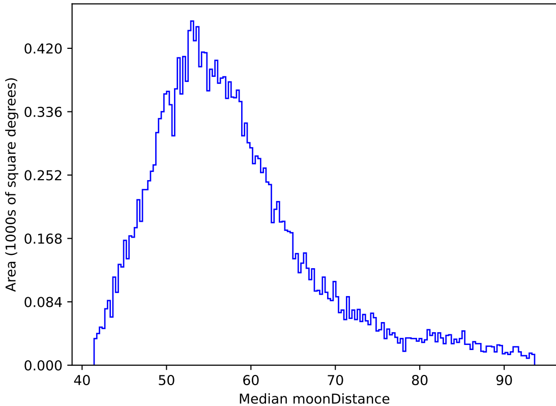
too_elab_r16_d3_giz_v3.4_10yrs All sky y band: Median moonDistance
