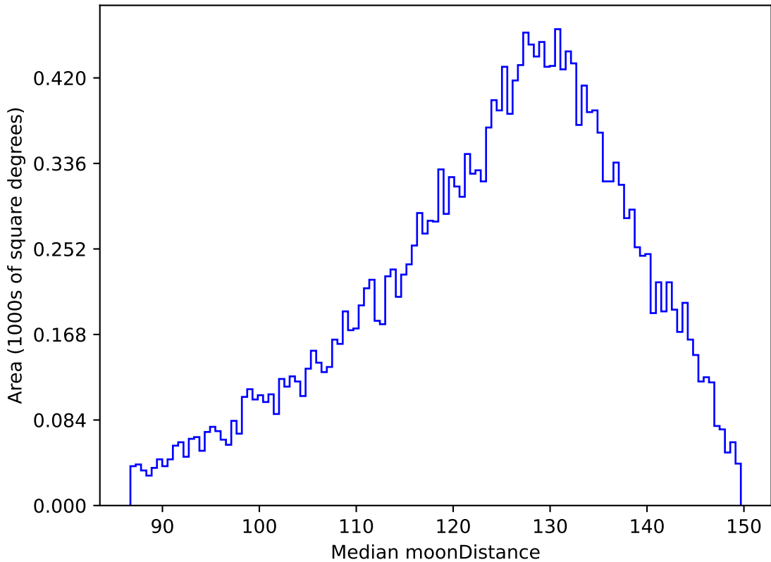
too_elab_r16_d3_giz_v3.4_10yrs All sky u band: Median moonDistance
