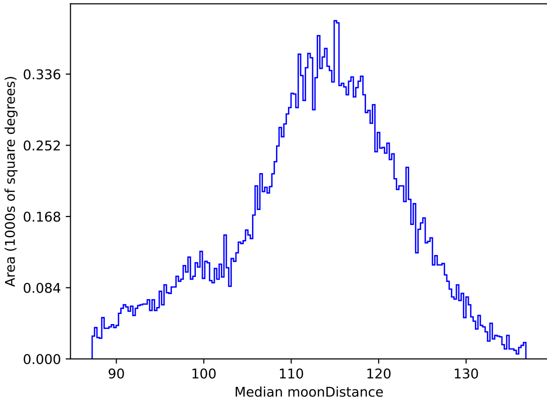
too_elab_r16_d3_giz_v3.4_10yrs All sky r band: Median moonDistance
