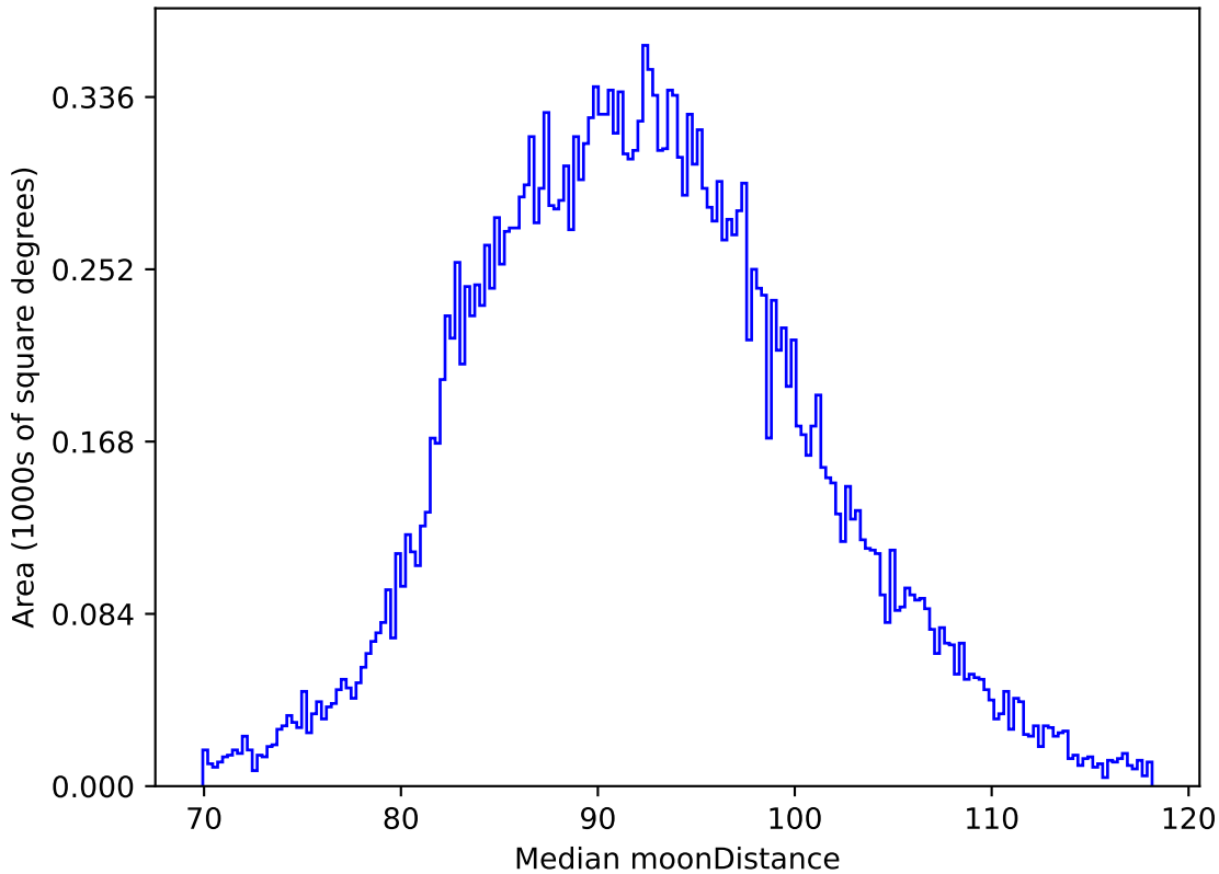
too_elab_r16_d3_giz_v3.4_10yrs All sky i band: Median moonDistance
