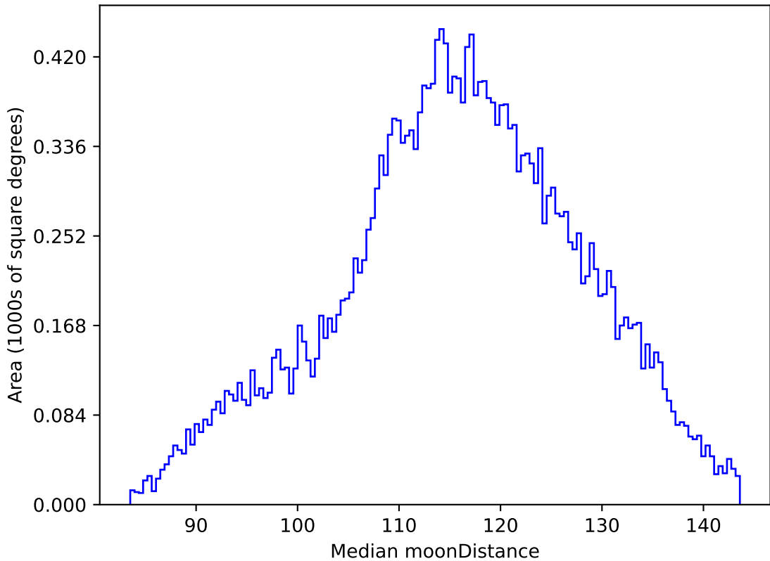
too_elab_r16_d3_giz_v3.4_10yrs All sky g band: Median moonDistance
