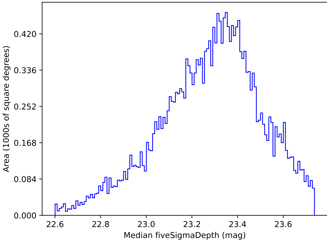
too_elab_r16_d3_giz_v3.4_10yrs Yr 1 u band: Median fiveSigmaDepth
