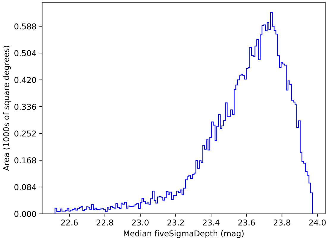
too_elab_r16_d3_giz_v3.4_10yrs Yr 1 i band: Median fiveSigmaDepth
