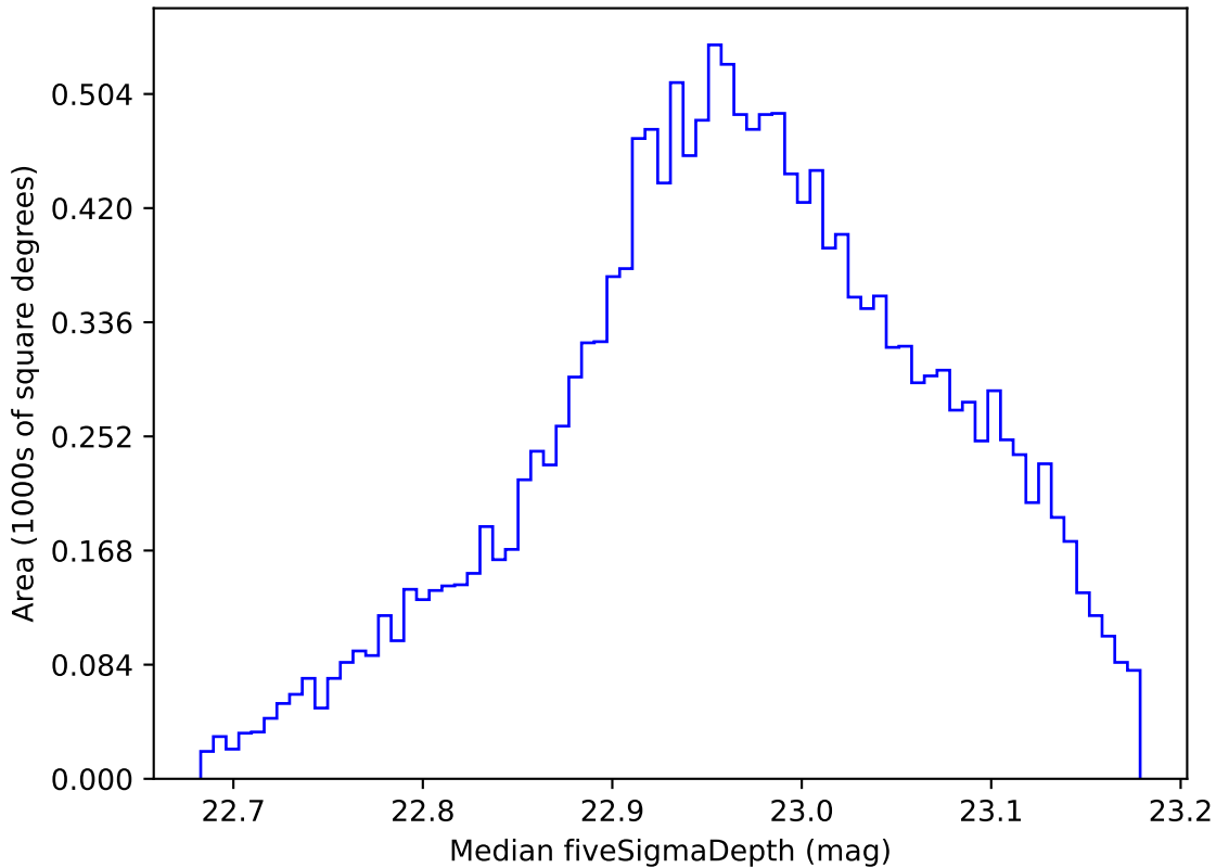
too_elab_r16_d3_giz_v3.4_10yrs WFD z band: Median fiveSigmaDepth
