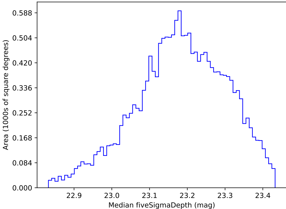
too_elab_r16_d3_giz_v3.4_10yrs WFD u band: Median fiveSigmaDepth
