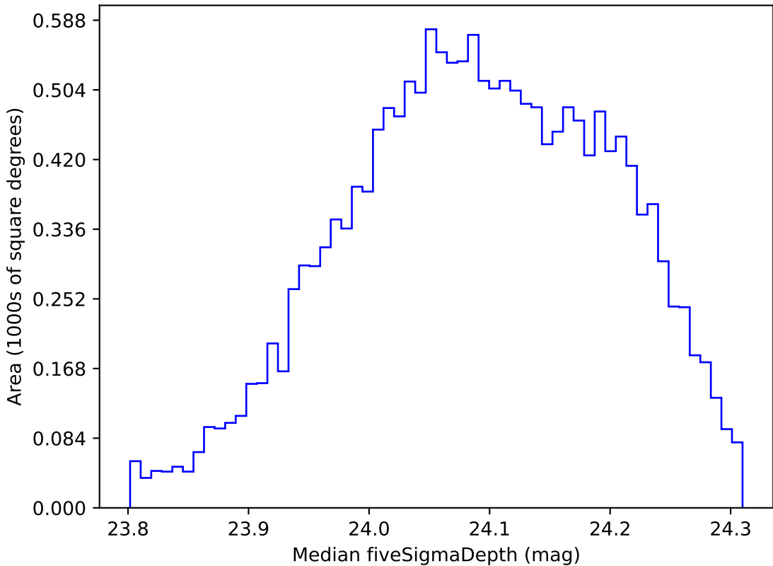
too_elab_r16_d3_giz_v3.4_10yrs WFD r band: Median fiveSigmaDepth
