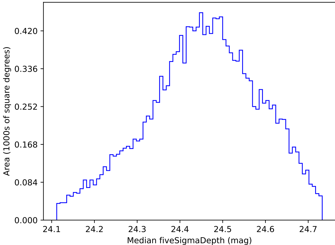
too_elab_r16_d3_giz_v3.4_10yrs WFD g band: Median fiveSigmaDepth
