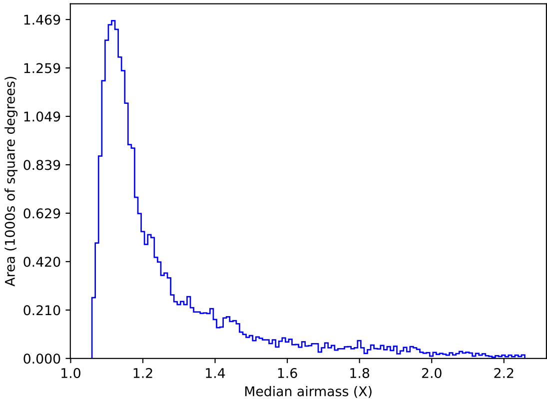
too_elab_r16_d3_giz_v3.4_10yrs Yr 1 z band: Median airmass
