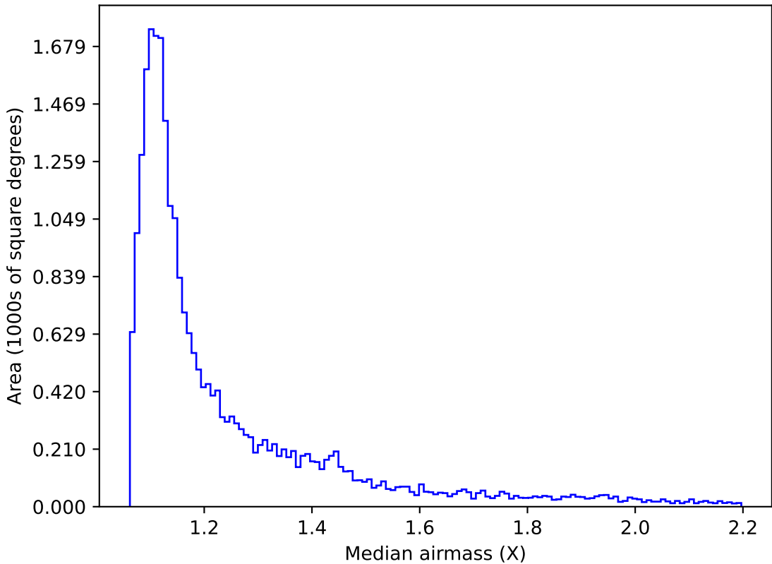
too_elab_r16_d3_giz_v3.4_10yrs Yr 1 i band: Median airmass
