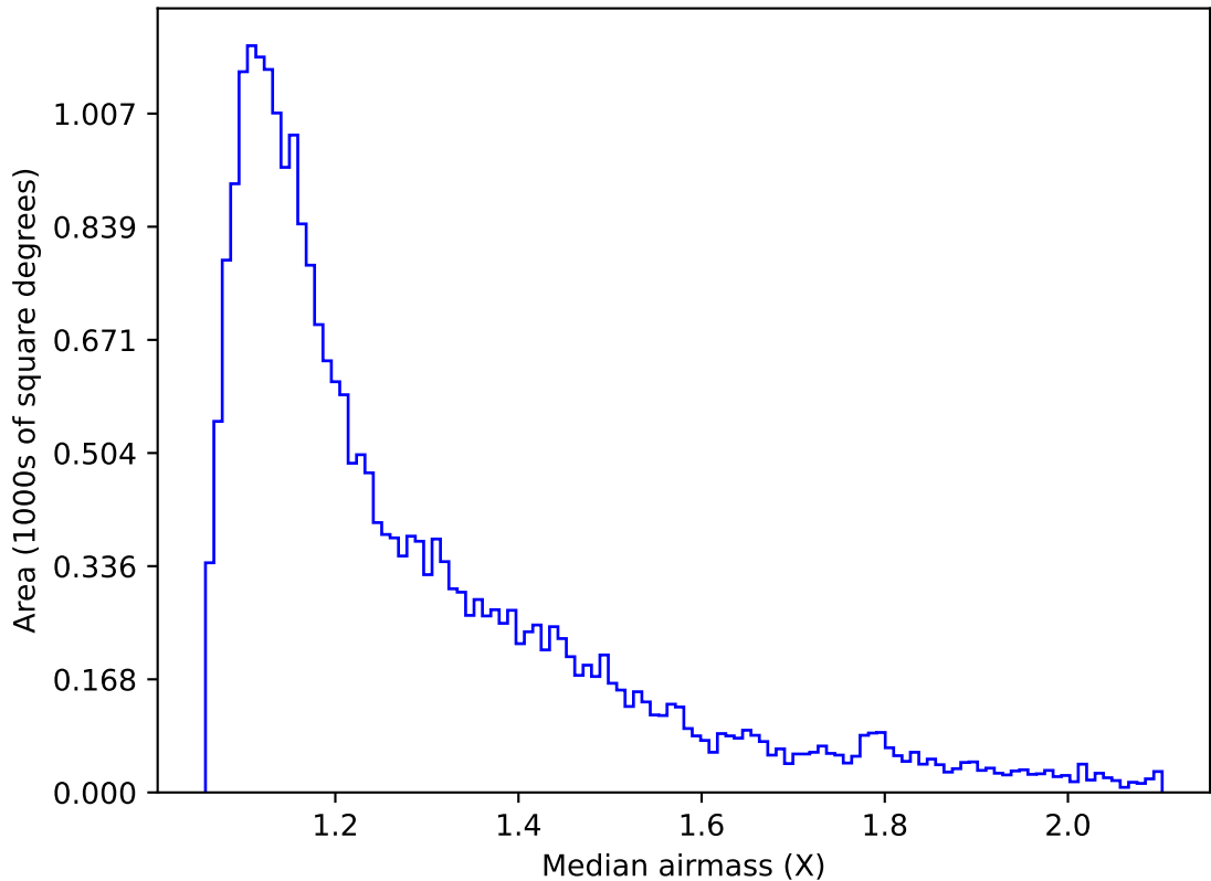
too_elab_r16_d3_giz_v3.4_10yrs Yr 1 g band: Median airmass
