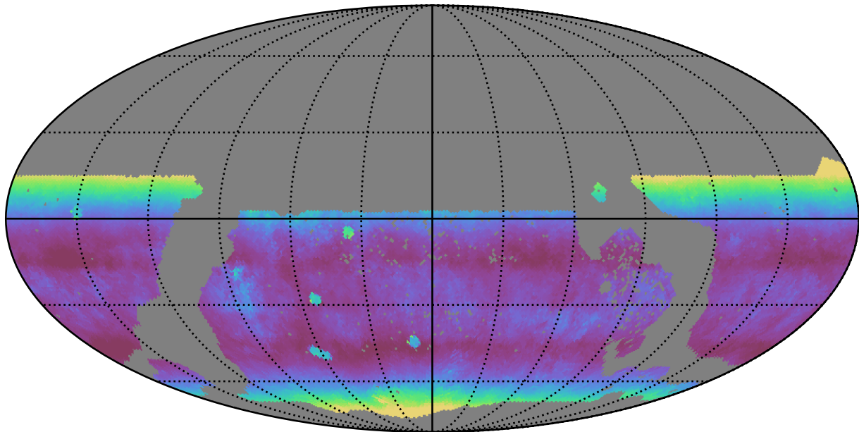
too_elab_r16_d3_giz_v3.4_10yrs WFD z band: Median airmass
