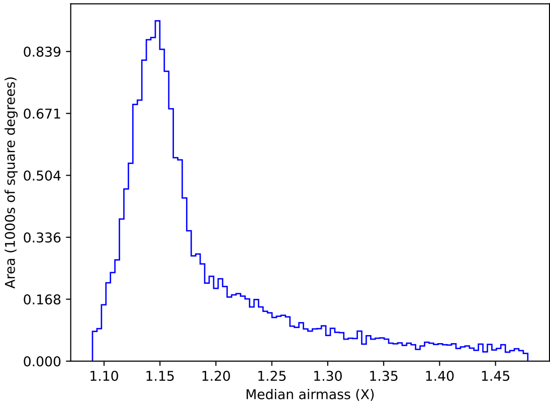
too_elab_r16_d3_giz_v3.4_10yrs WFD y band: Median airmass
