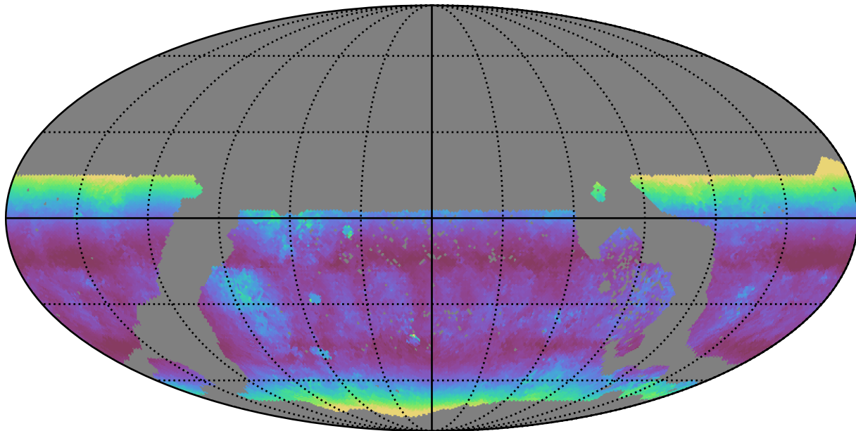
too_elab_r16_d3_giz_v3.4_10yrs WFD u band: Median airmass
