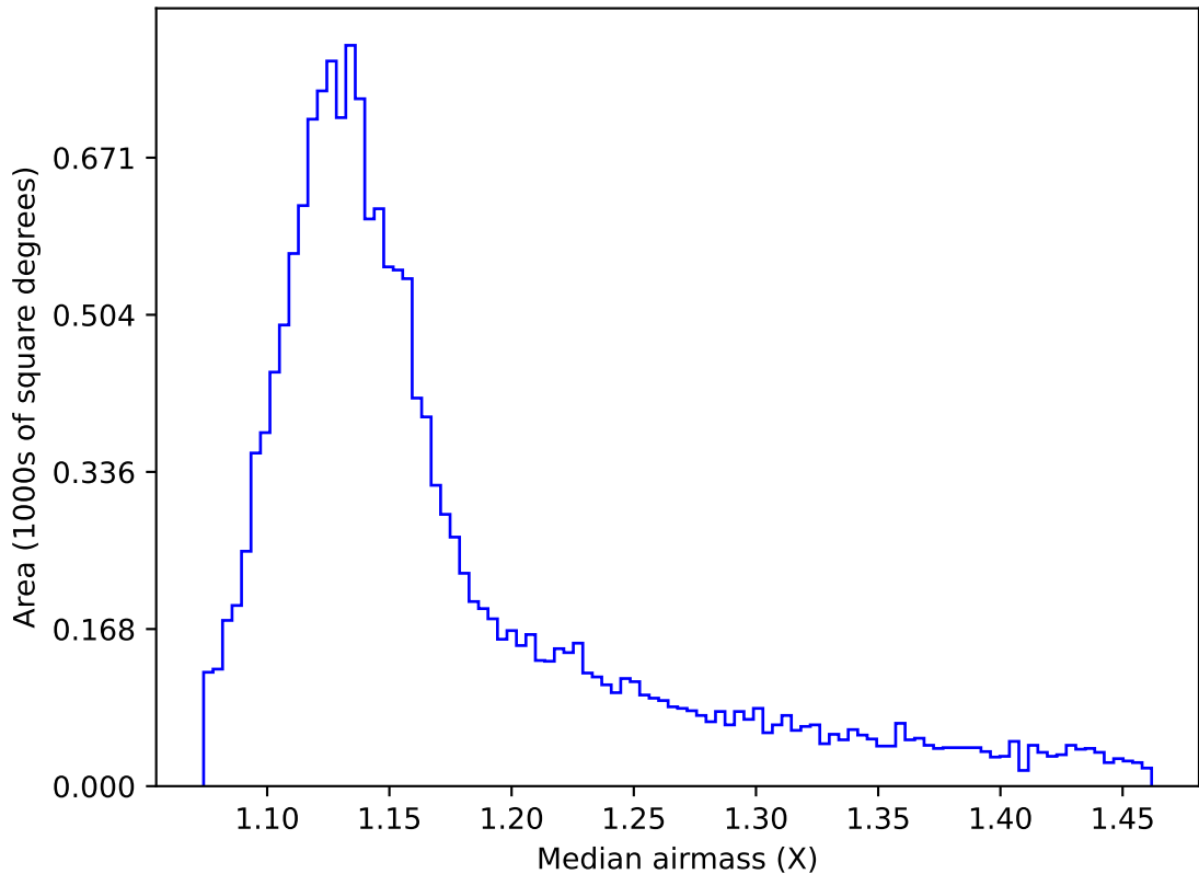
too_elab_r16_d3_giz_v3.4_10yrs WFD r band: Median airmass
