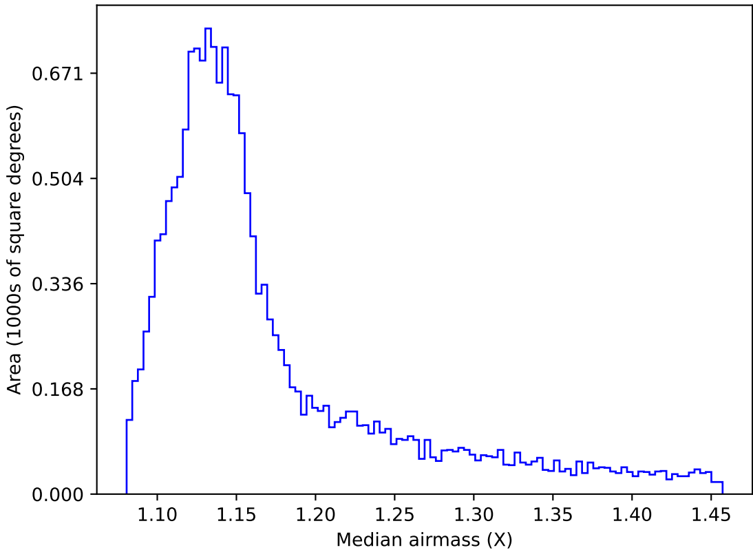
too_elab_r16_d3_giz_v3.4_10yrs WFD i band: Median airmass
