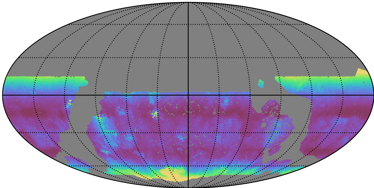
too_elab_r16_d3_giz_v3.4_10yrs WFD g band: Median airmass
