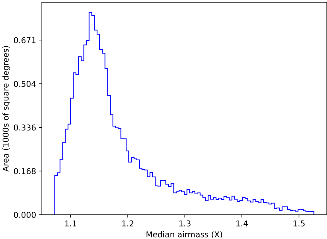
too_elab_r16_d3_giz_v3.4_10yrs WFD g band: Median airmass
