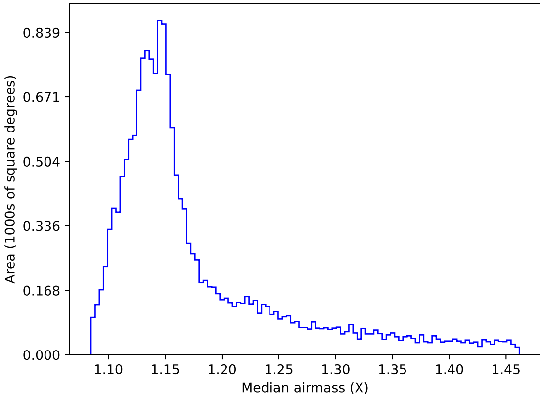
too_elab_r16_d3_giz_v3.4_10yrs WFD all bands: Median airmass
