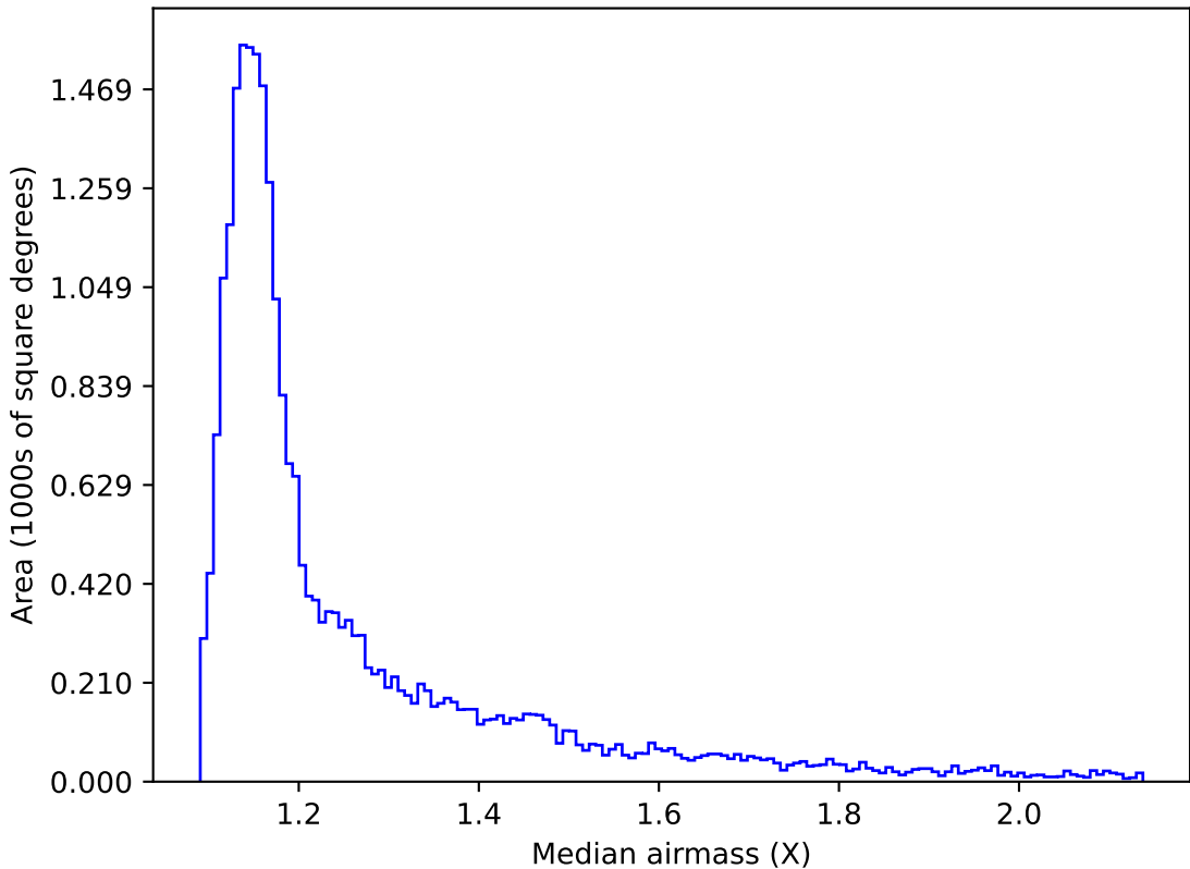
too_elab_r16_d3_giz_v3.4_10yrs All sky z band: Median airmass
