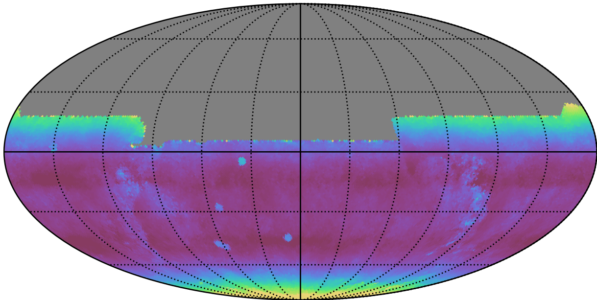
too_elab_r16_d3_giz_v3.4_10yrs All sky y band: Median airmass
