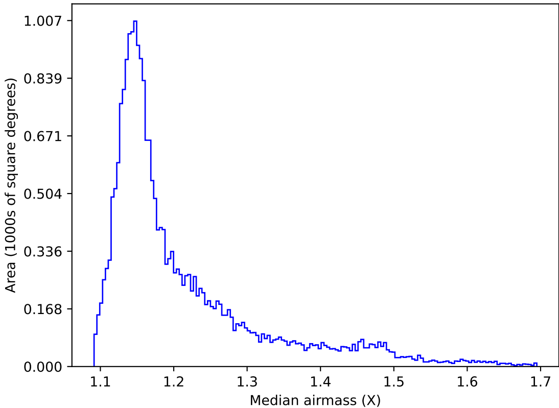
too_elab_r16_d3_giz_v3.4_10yrs All sky y band: Median airmass
