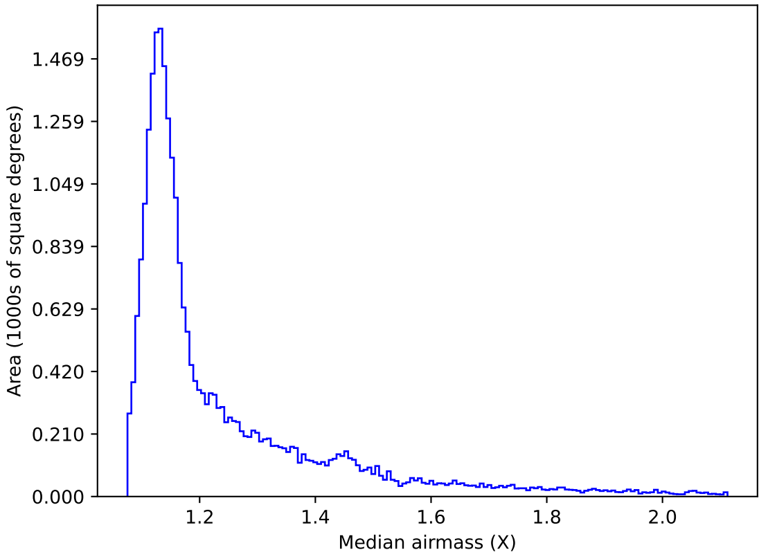
too_elab_r16_d3_giz_v3.4_10yrs All sky r band: Median airmass
