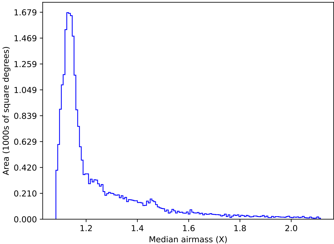
too_elab_r16_d3_giz_v3.4_10yrs All sky i band: Median airmass
