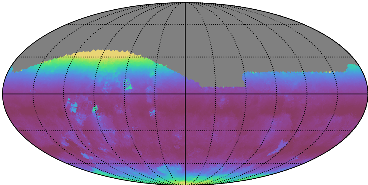
too_elab_r16_d3_giz_v3.4_10yrs All sky g band: Median airmass
