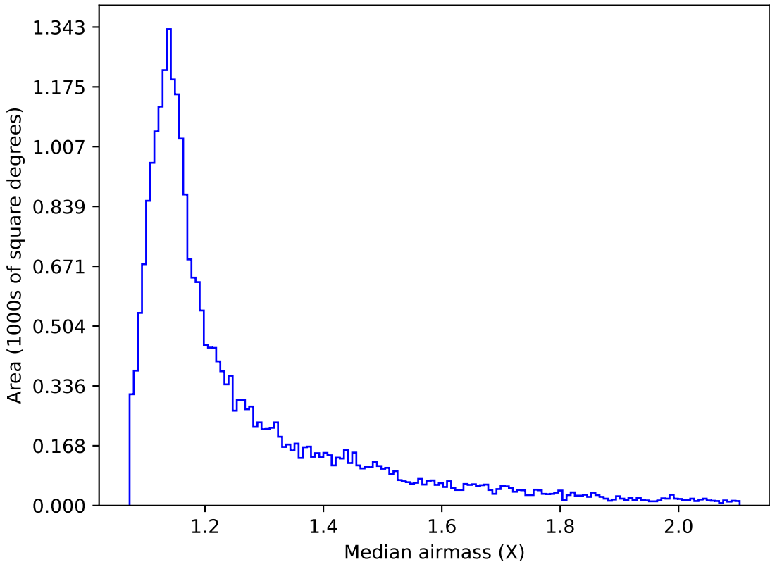
too_elab_r16_d3_giz_v3.4_10yrs All sky g band: Median airmass
