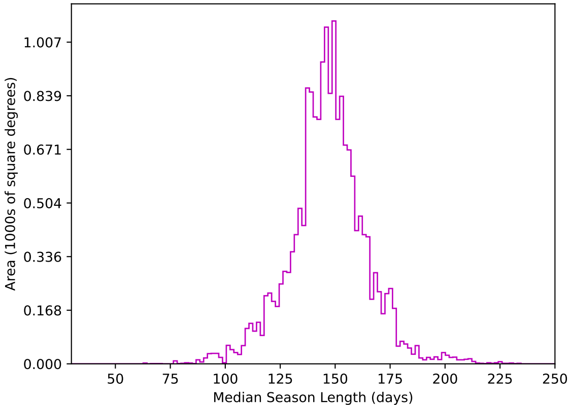
too_elab_r16_d3_giz_v3.4_10yrs WFD z band: Median Season Length
