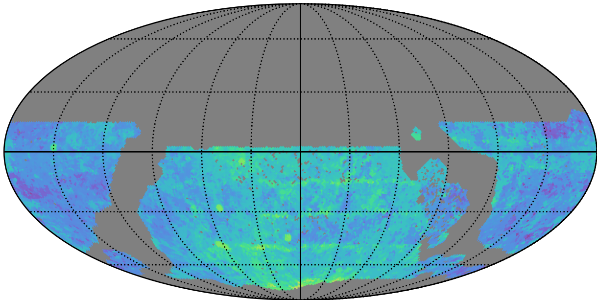
too_elab_r16_d3_giz_v3.4_10yrs WFD y band: Median Season Length
