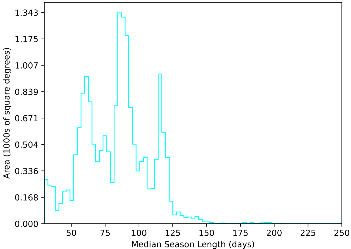
too_elab_r16_d3_giz_v3.4_10yrs WFD u band: Median Season Length
