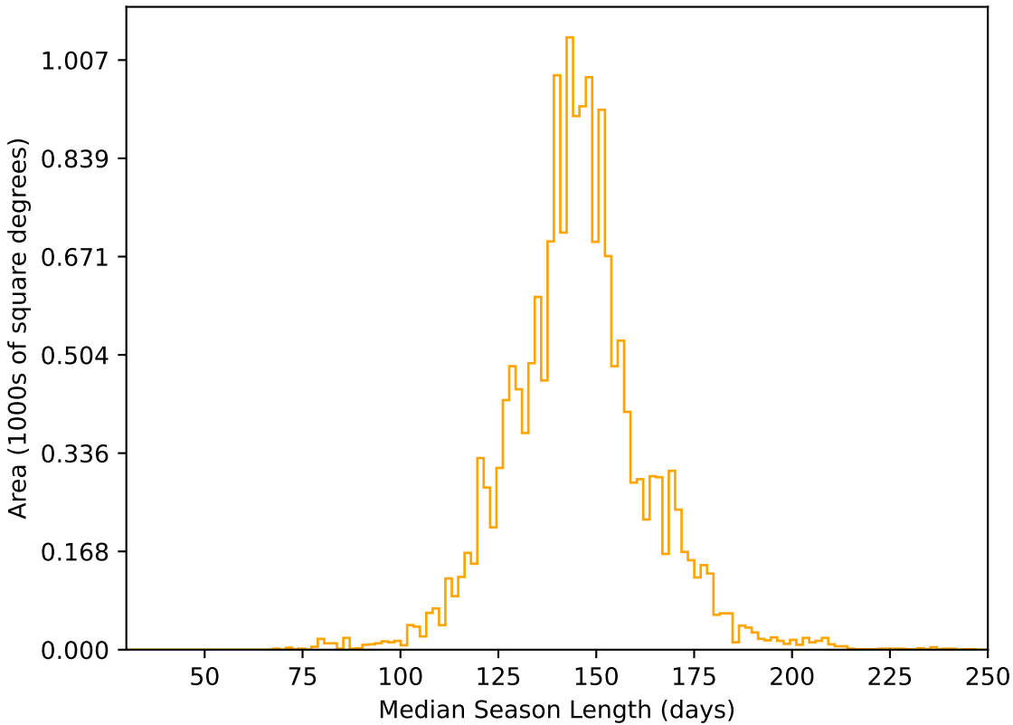
too_elab_r16_d3_giz_v3.4_10yrs WFD r band: Median Season Length
