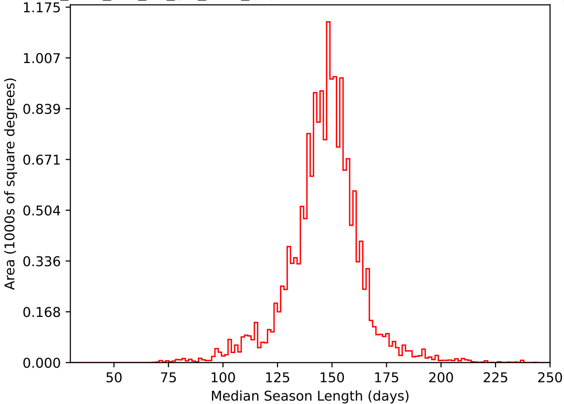
too_elab_r16_d3_giz_v3.4_10yrs WFD i band: Median Season Length
