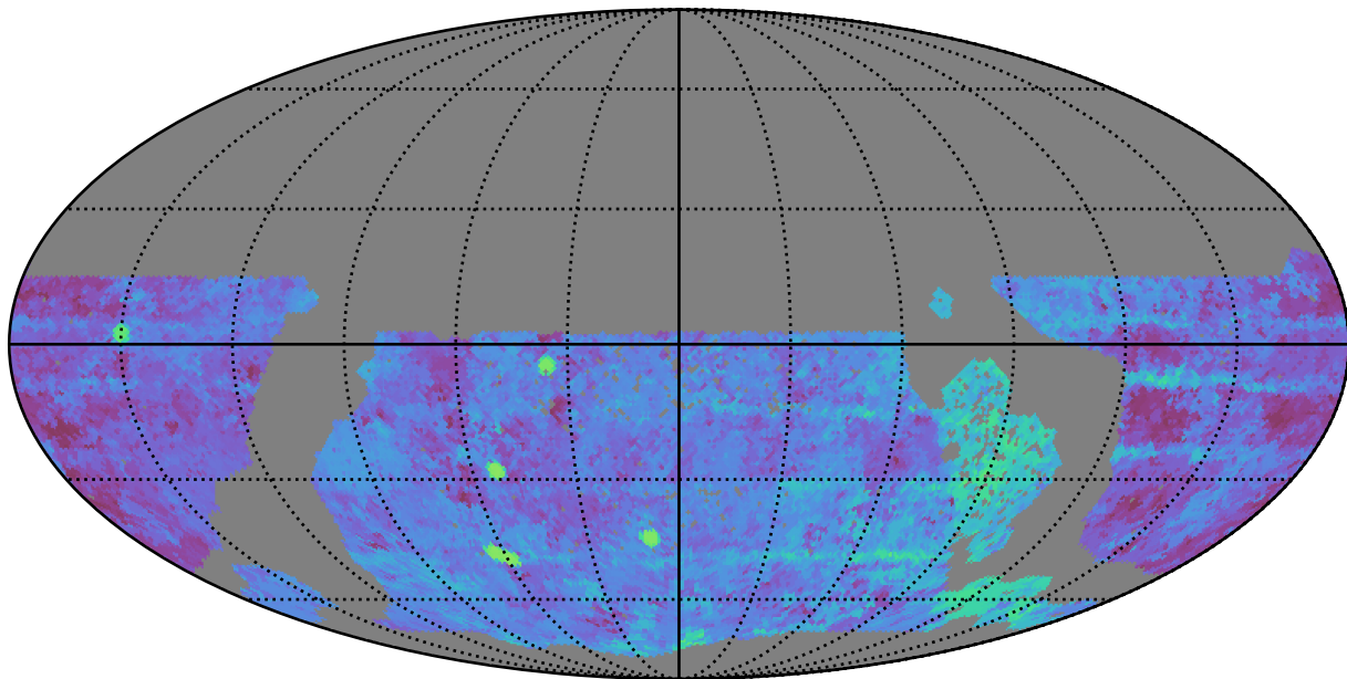
too_elab_r16_d3_giz_v3.4_10yrs WFD g band: Median Season Length
