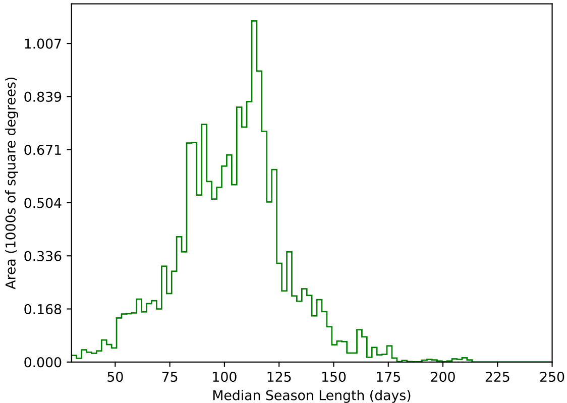
too_elab_r16_d3_giz_v3.4_10yrs WFD g band: Median Season Length
