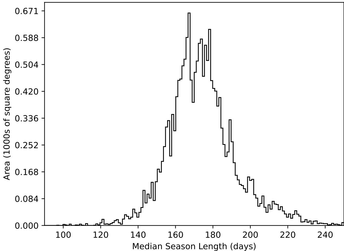
too_elab_r16_d3_giz_v3.4_10yrs WFD all bands: Median Season Length
