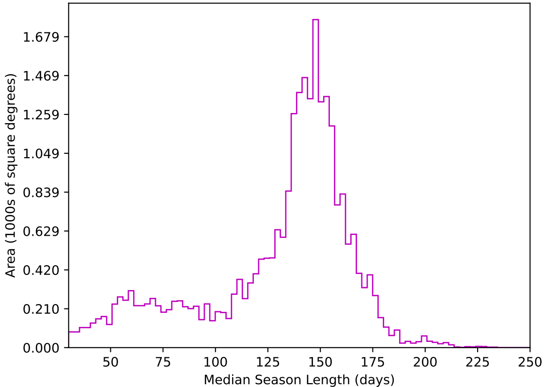
too_elab_r16_d3_giz_v3.4_10yrs All sky z band: Median Season Length
