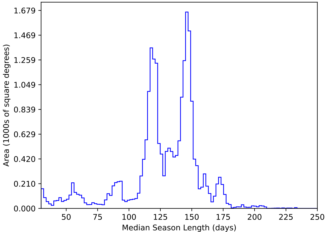
too_elab_r16_d3_giz_v3.4_10yrs All sky y band: Median Season Length
