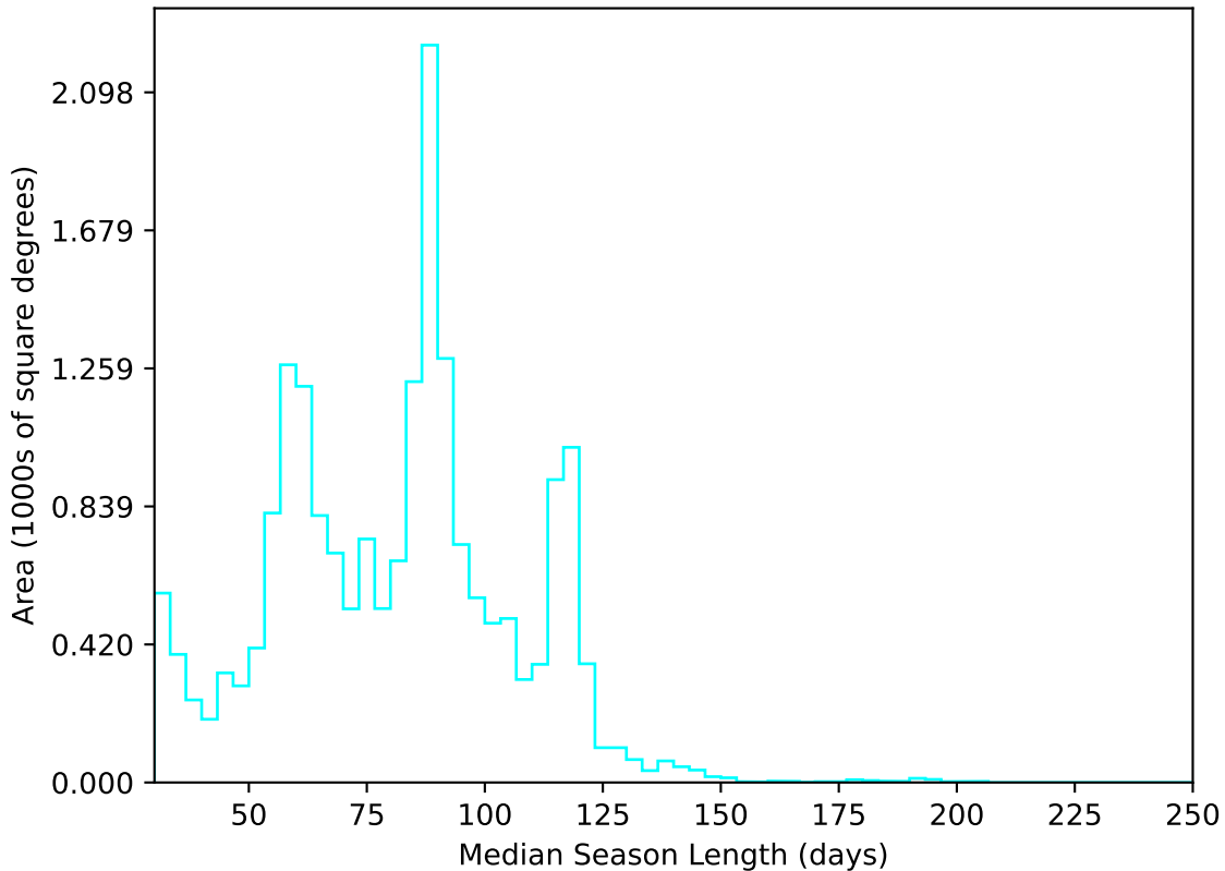
too_elab_r16_d3_giz_v3.4_10yrs All sky u band: Median Season Length
